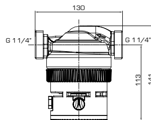
Laing Ecocirc® auto 20-130 G
