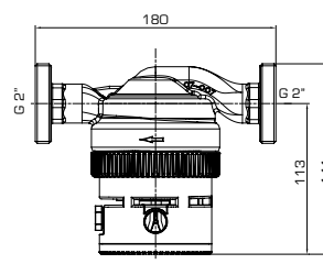
Laing Ecocirc® auto 32-180 G
